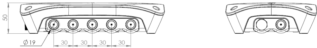
Figure 9 Side views showing 5 knock-outs for cables and the Gore-Tex type of membrane for ventilation
